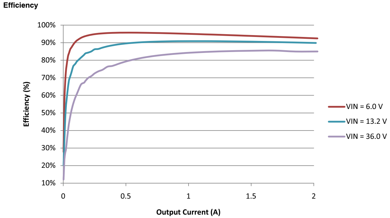
Figure 4. Efficiency at 170 kHz for a 5.0 V output
