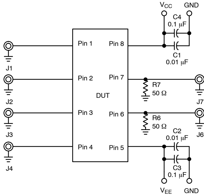
Figure 6. Configuration 3 Schematic
