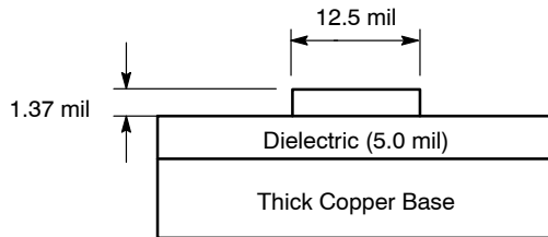
Figure 5. Board Stack-up
