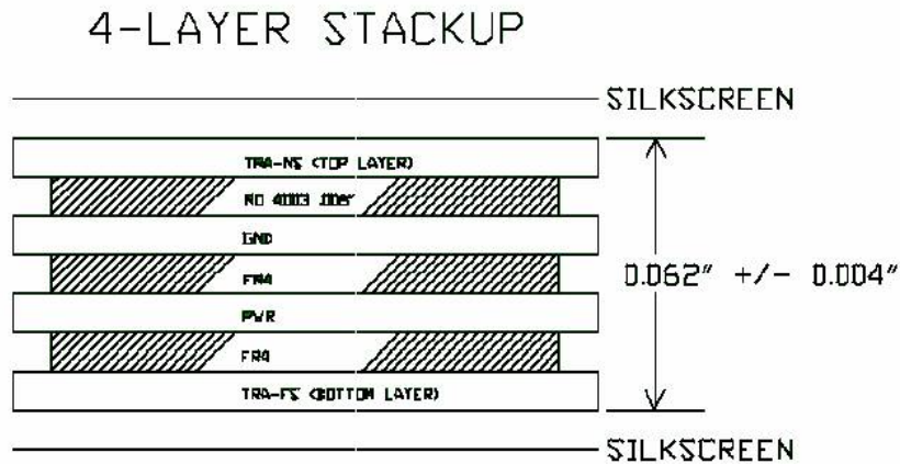
Figure 3. Evaluation Board Lay-up
