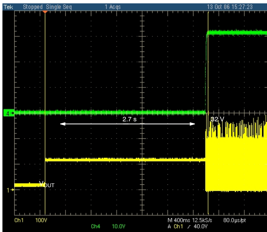
Figure 6. Start-up Time, V_{IN} = 85 \text{ Vac}
