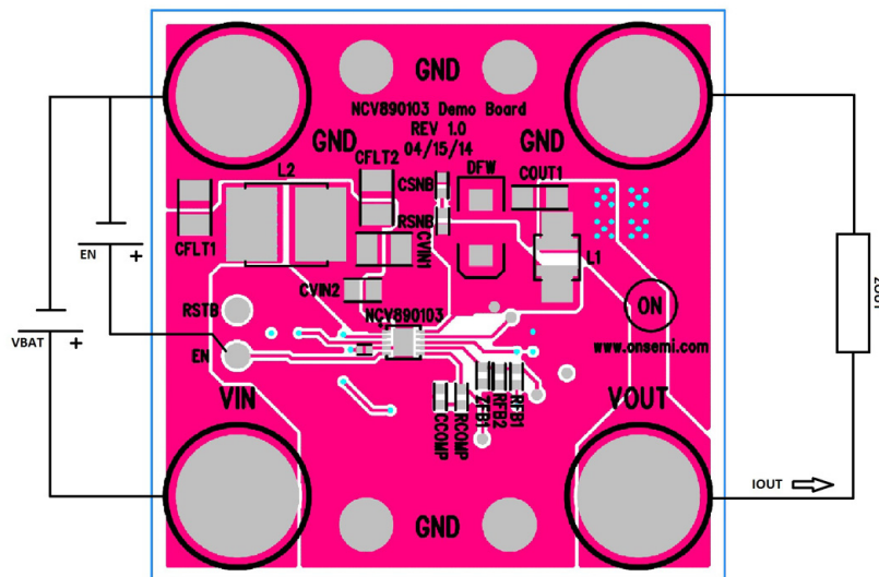
Figure 5. NCV890103 Board Connections
