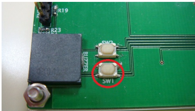
Figure 6. Reset Switch of LC717A10AR and LC898301XA
