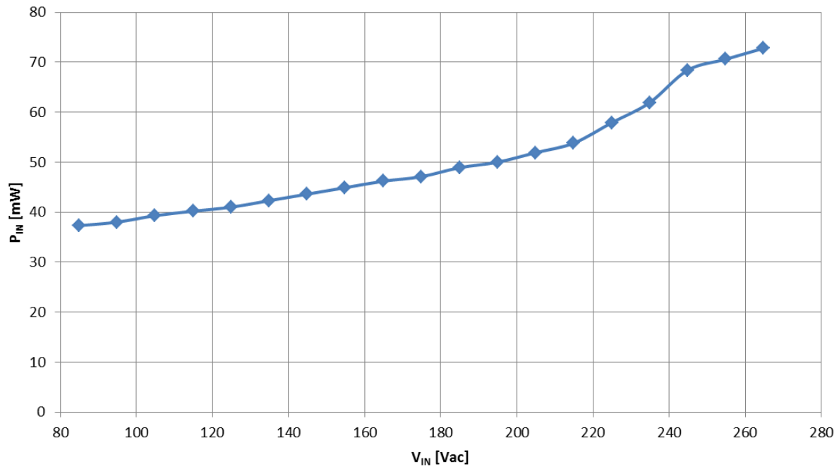
Figure 6. No-load Power Consumption vs. Line Input Curves
