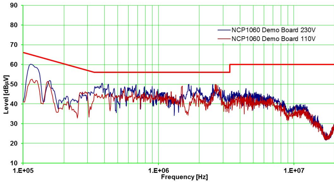
Figure 4. Conducted Emission Quasi-peak dB \mu V (Domestic)
