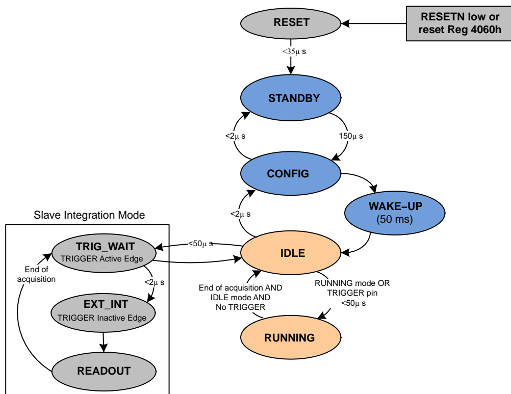
Figure 12. Sensor State Diagram
