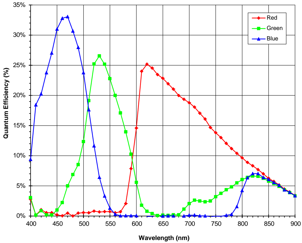
Figure 5. Nominal KAI-0330-CBA Spectral Response
