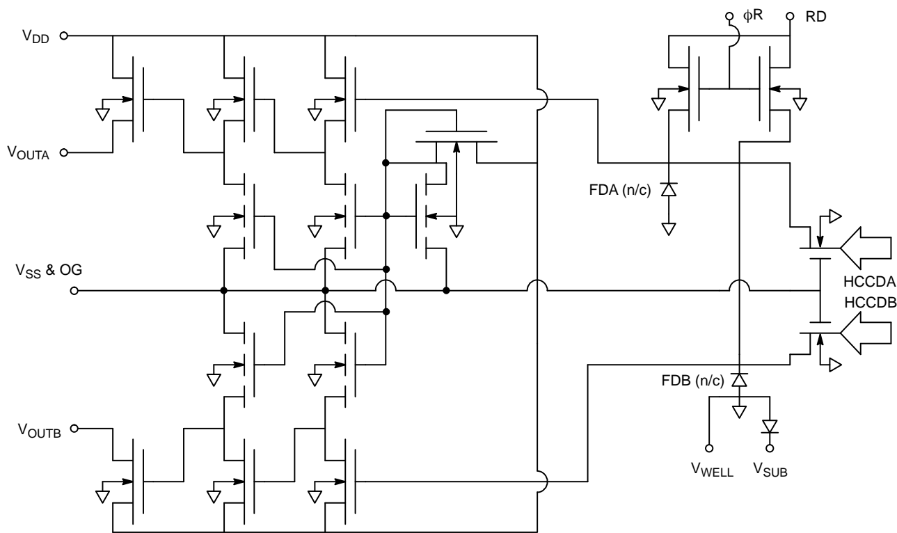
Figure 3. Output Structure
