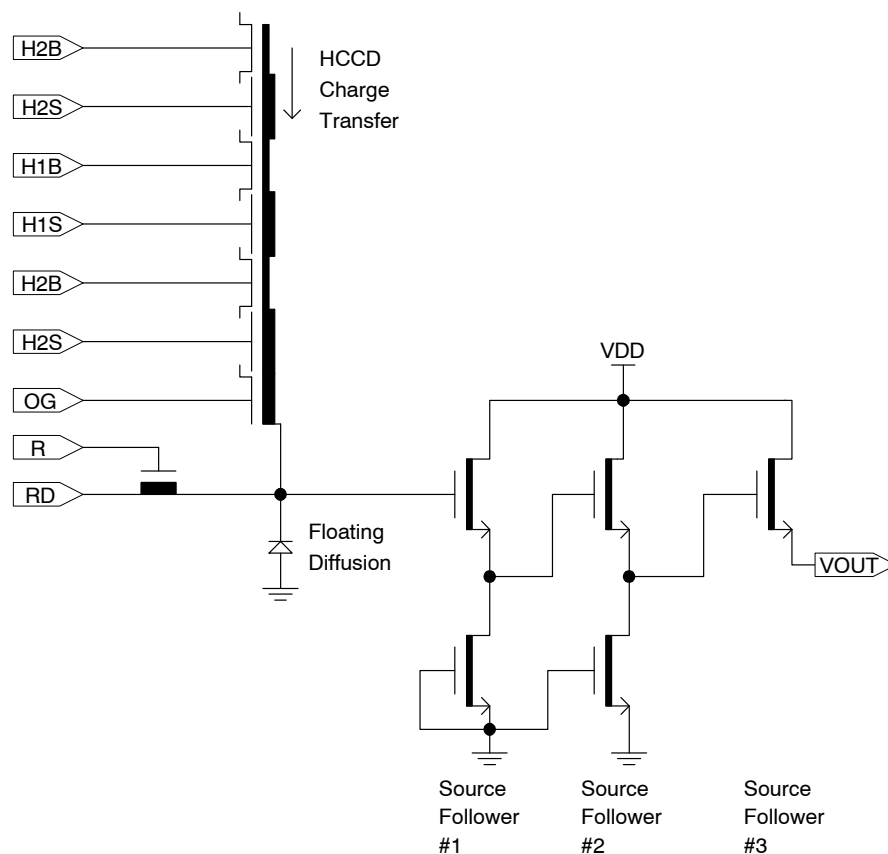
Figure 7. Output Architecture
