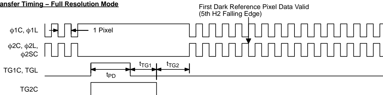
Figure 24. Timing Diagram
