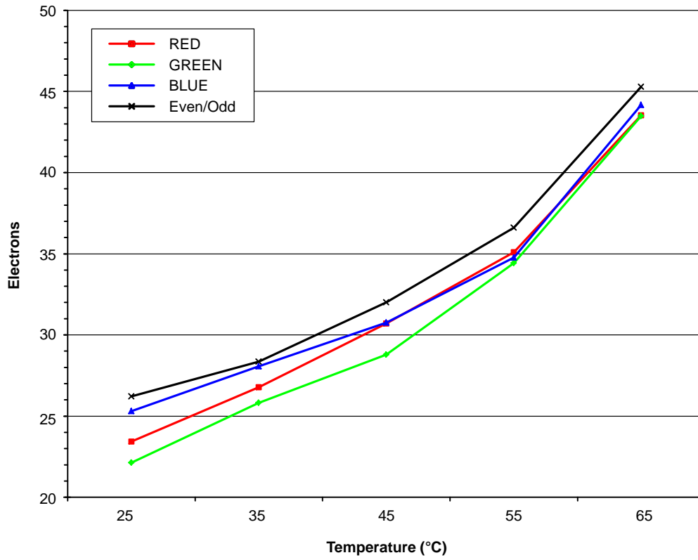
Figure 14. Dark Noise vs. Temperature
