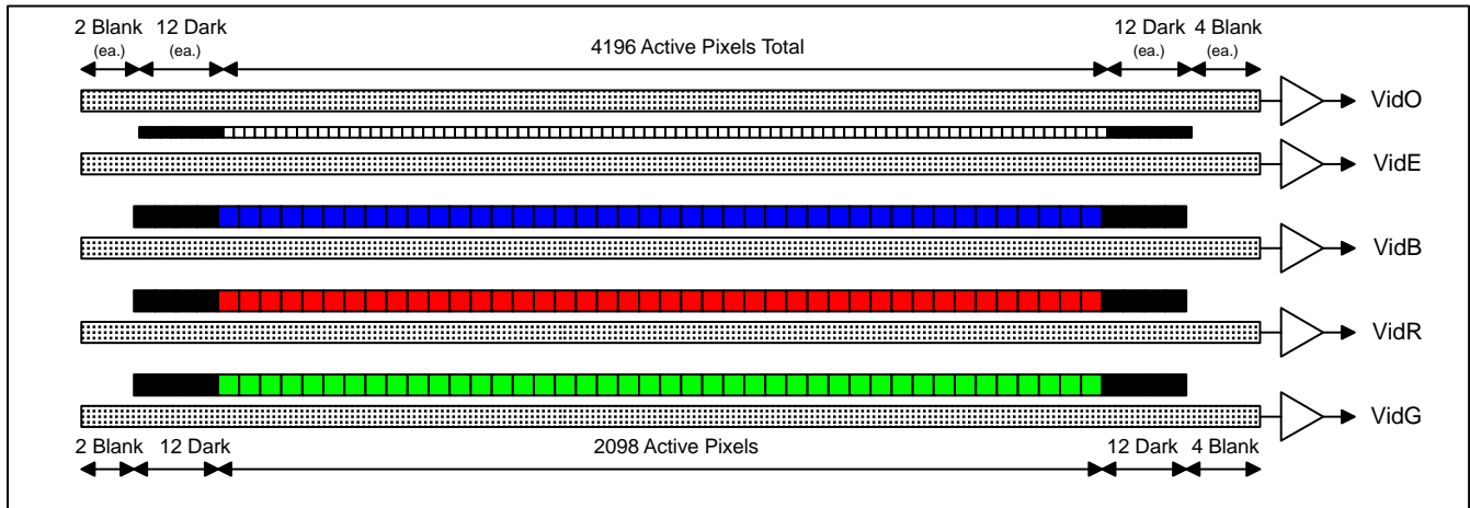
Figure 2. Block Diagram
