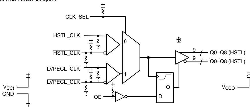
Figure 3. Logic Diagram
