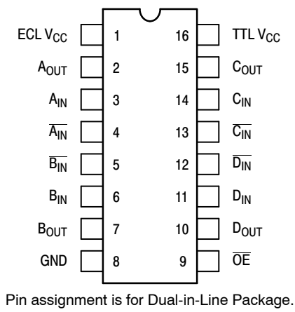
Figure 2. Dip Pin Assignment
