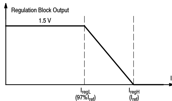
Figure 25. Regulation Characteristic
