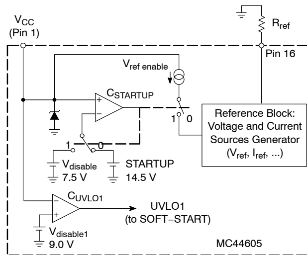
Figure 3. V CC Management
