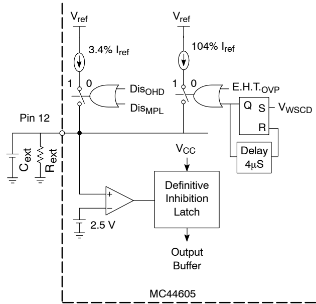
Figure 15. Disabling Block
