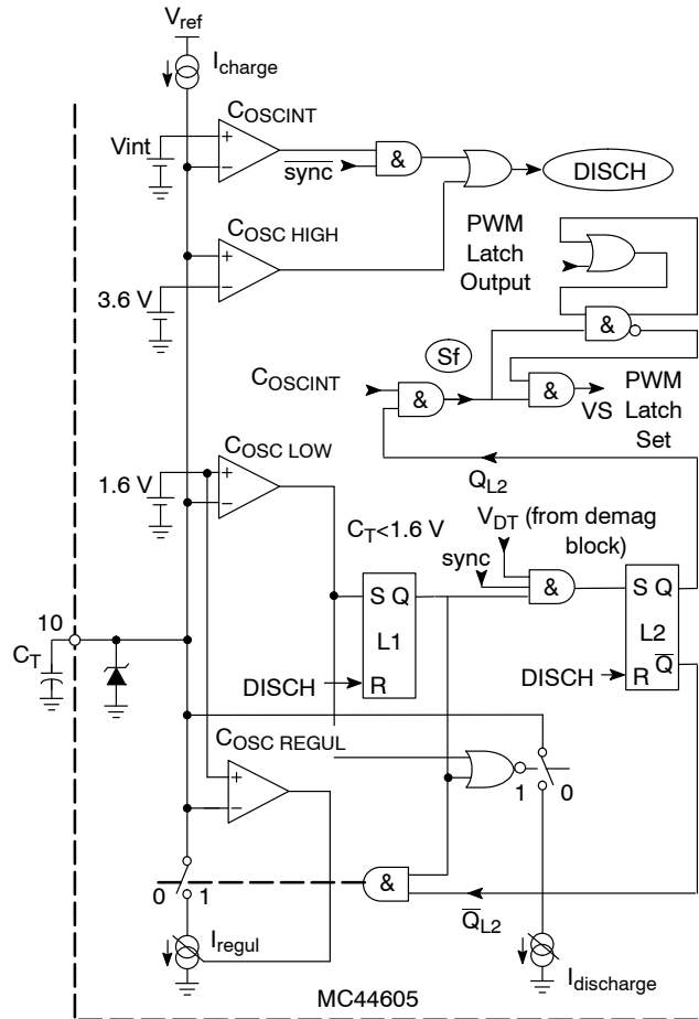
Figure 5. Oscillator
