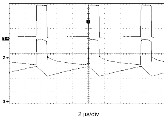
Figure 42. NCP1402SN30T1 Operating Waveforms (Heavy Load)
