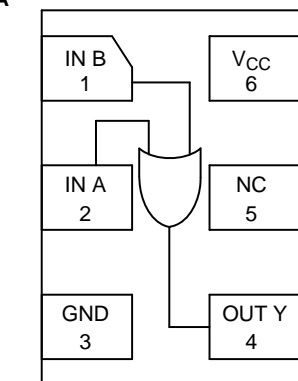
Figure 1. Pinouts (Top View)
