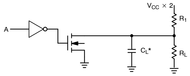
Figure 4. Test Circuit
