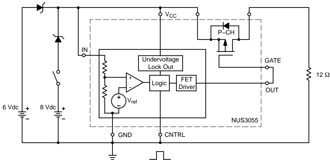
Figure 11. Test Circuit for T_{ON CT} and T_{OFF CT}
