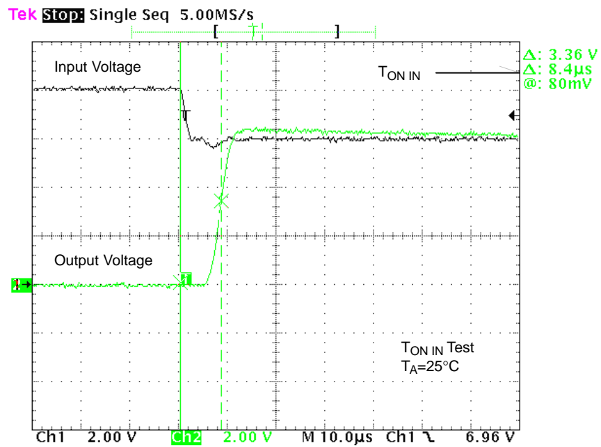
Figure 9. T_{ON\ IN} Waveforms
