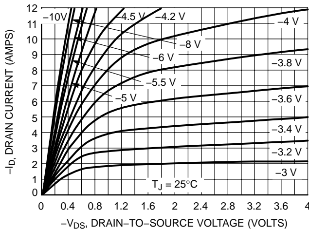
Figure 4. On-Region Characteristics
