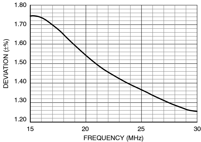
Figure 2. Deviation vs. Frequency ( V_{DD} = 1.6\text{ V} - 2.0\text{ V} )
