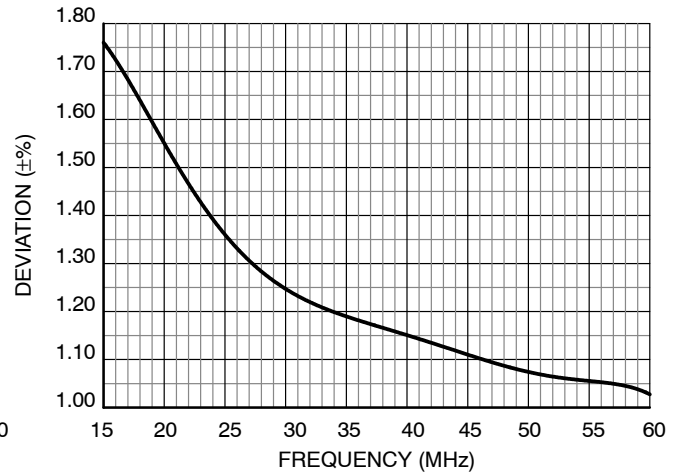
Figure 3. Deviation vs. Frequency ( V_{DD} = 2.3\text{ V} - 3.6\text{ V} )
