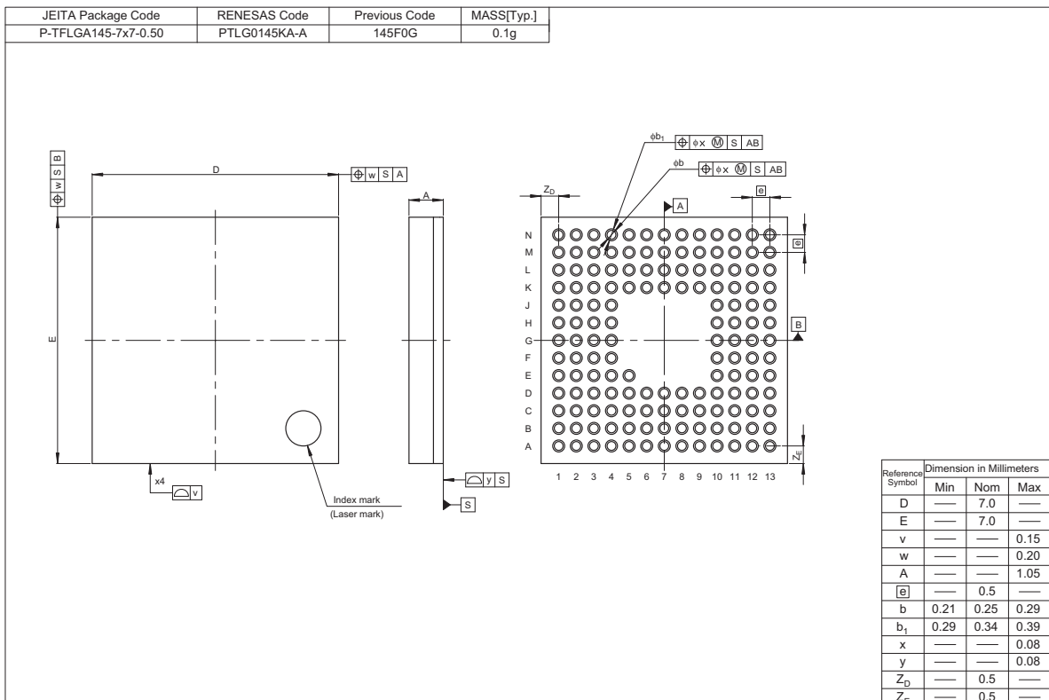
Figure 1.4 145-pin LGA
