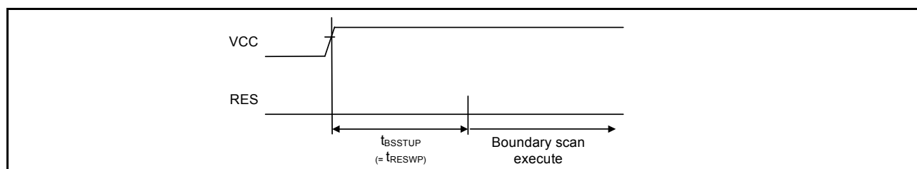
Figure 2.97 Boundary scan circuit startup timing
