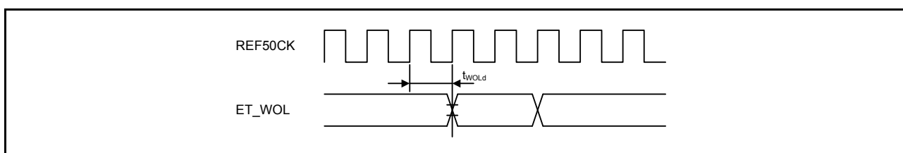
Figure 2.63 WOL output timing for RMII
