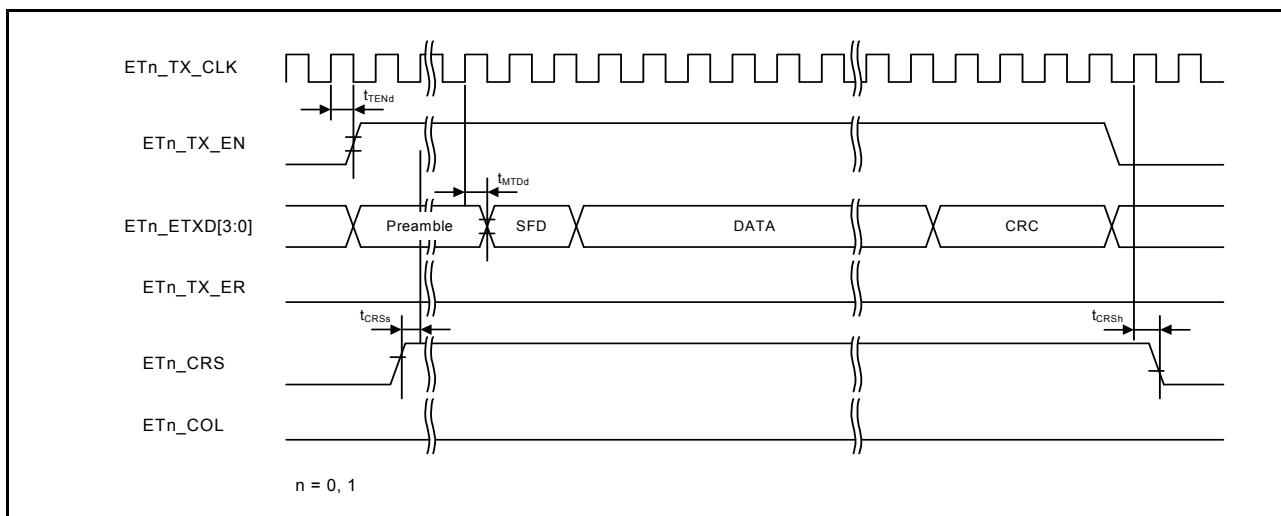
Figure 2.64 MII transmission timing in normal operation
