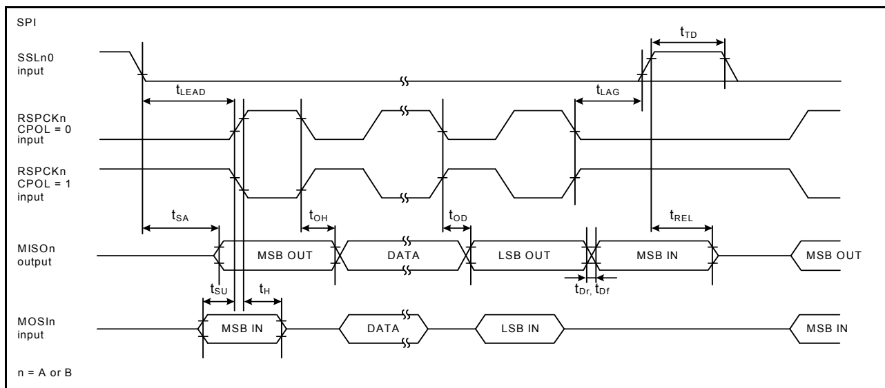
Figure 2.49 SPI timing for slave when CPHA = 0
