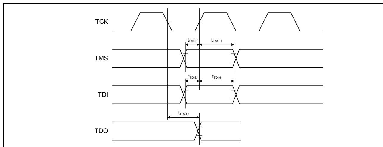
Figure 2.96 Boundary scan input/output timing
