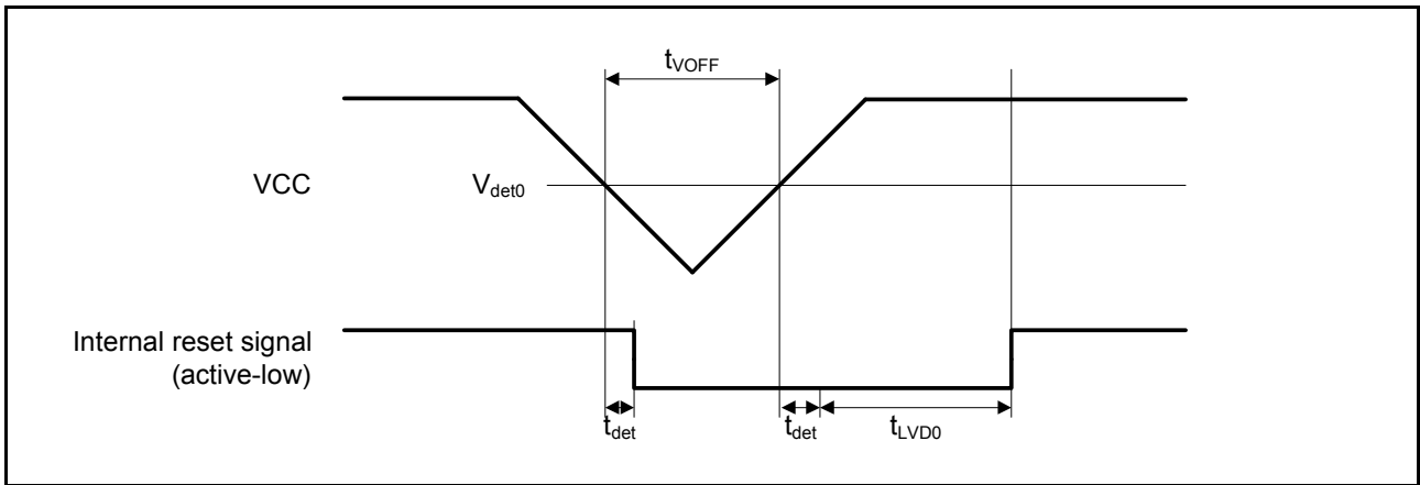
Figure 2.90 Voltage detection circuit timing ( V_{det0} )
