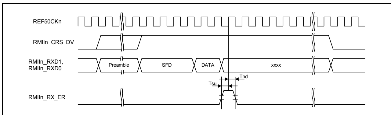
Figure 2.62 RMII reception timing when an error occurs
