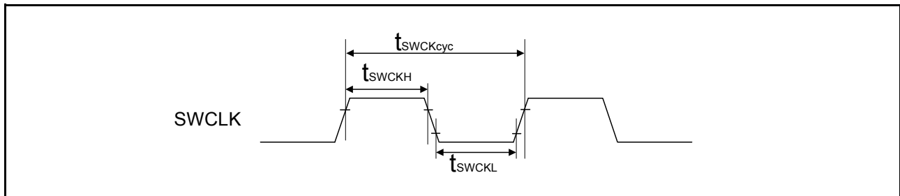
Figure 2.100 SWD SWCLK timing
