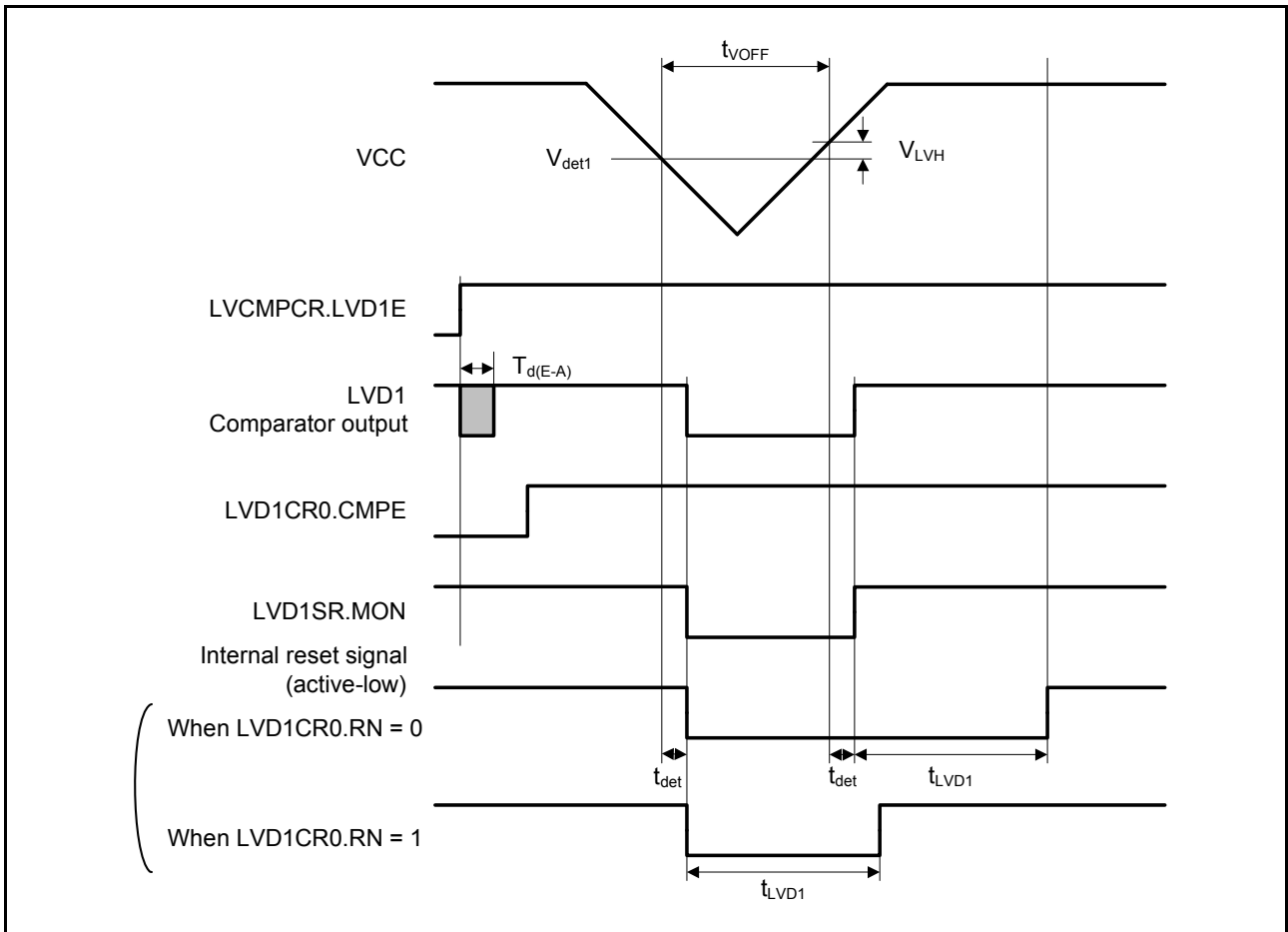
Figure 2.91 Voltage detection circuit timing ( V_{det1} )
