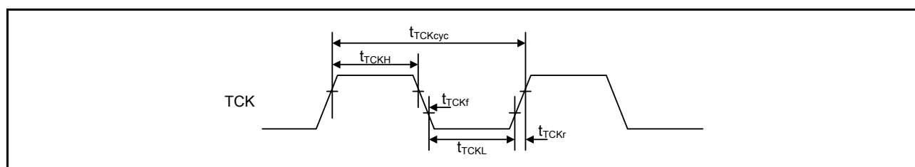
Figure 2.95 Boundary scan TCK timing
