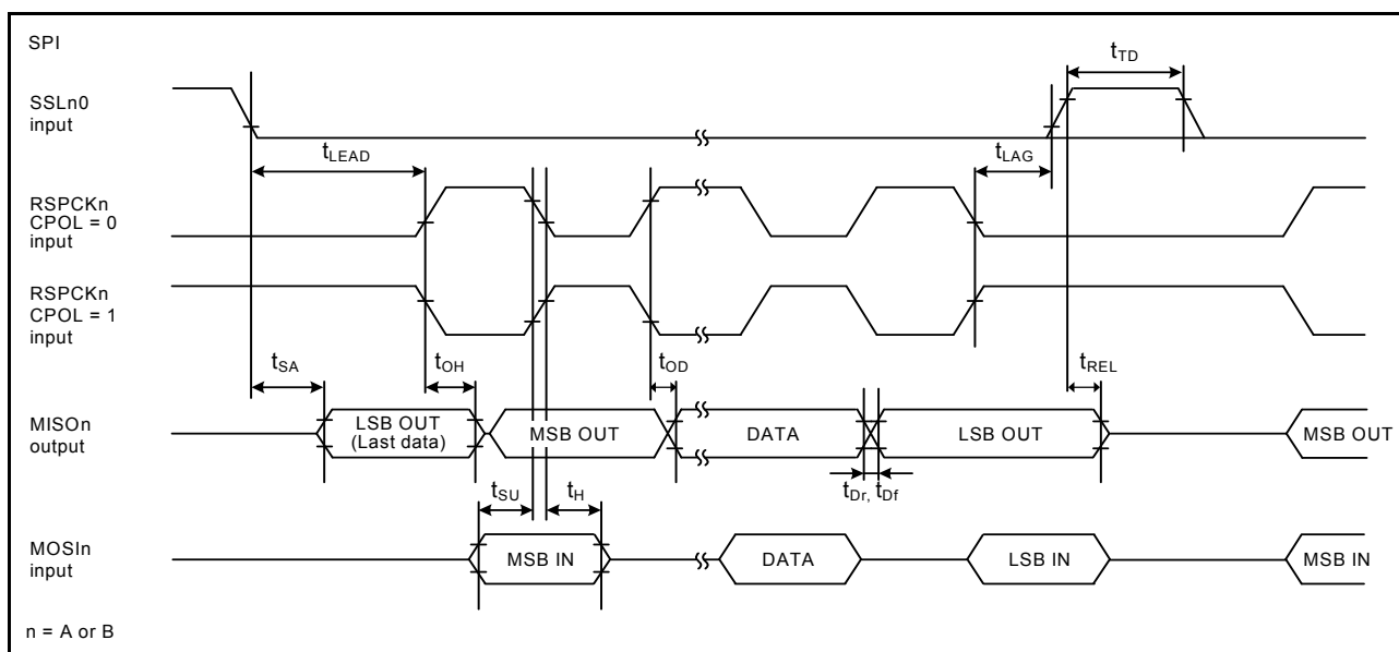
Figure 2.50 SPI timing for slave when CPHA = 1
