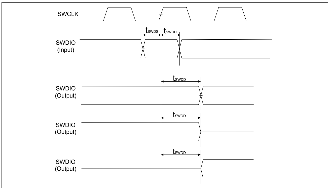
Figure 2.101 SWD input/output timing
