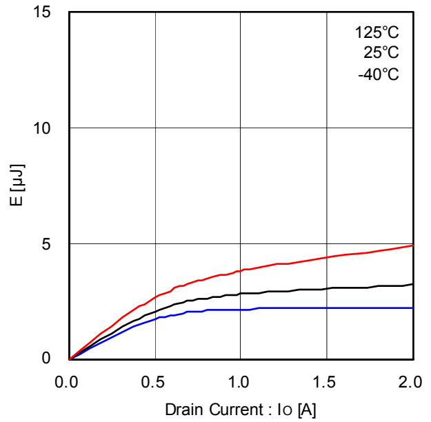
Figure 23. High Side Recovery Loss (VDC=150V)
