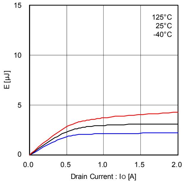
Figure 25. Low Side Recovery Loss (VDC=150V)
