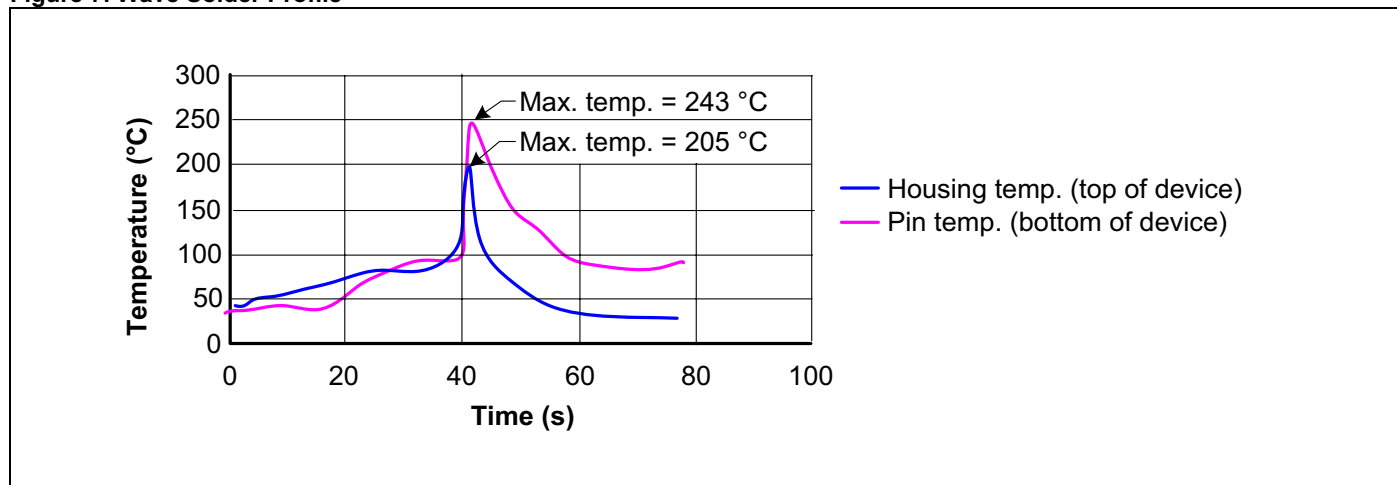
Figure 7. Wave Solder Profile
