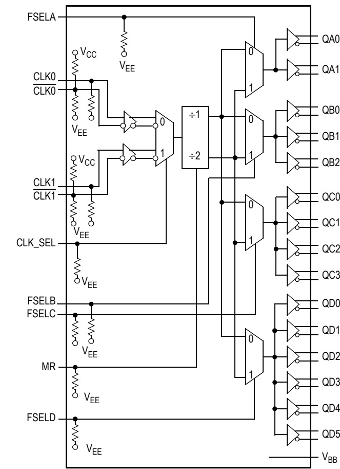
Figure 1. MC100ES6222 Logic Diagram
