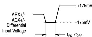
Figure 39. ARX/ACX Timing
