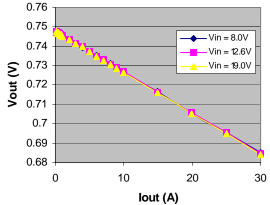
FIGURE 12. DEEPER SLEEP MODE LOAD LINE, 2 PHASE, DCM OPERATION, PSi# = LOW, VID = 0.75V
