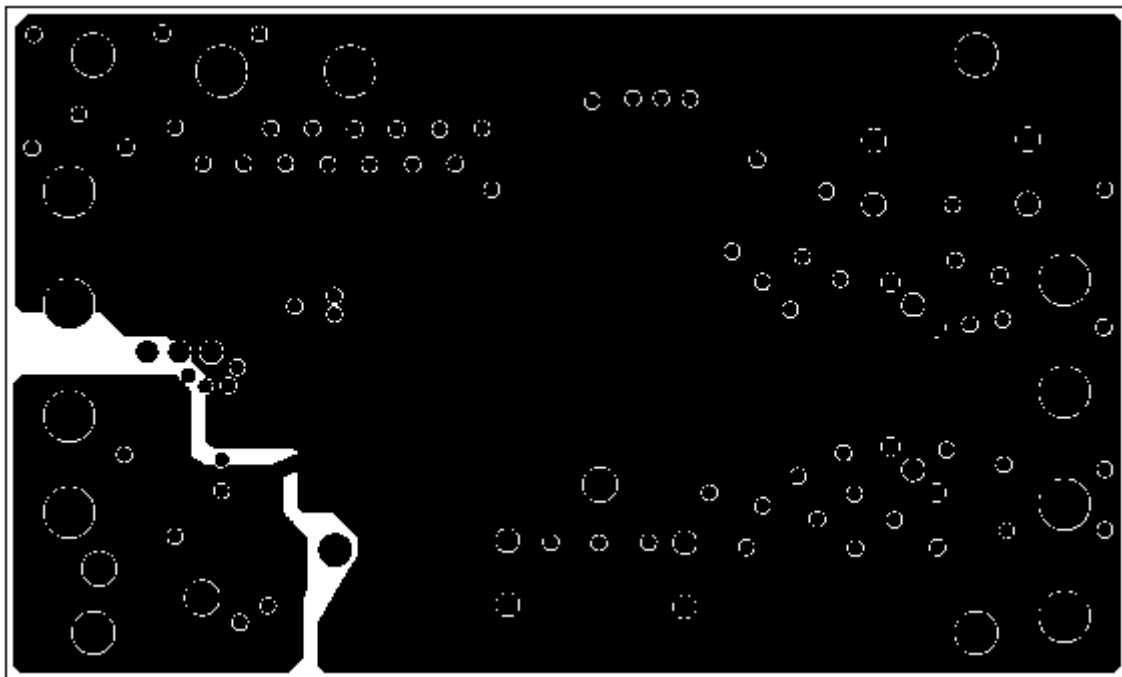
FIGURE 9. TOP LAYER 2
