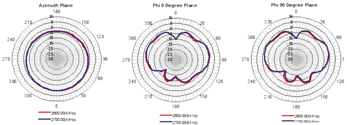
2400-2700 MHz Band
