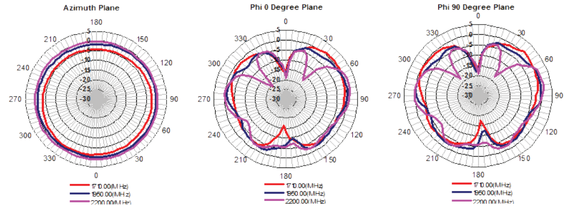
1710-2200 MHz Band
