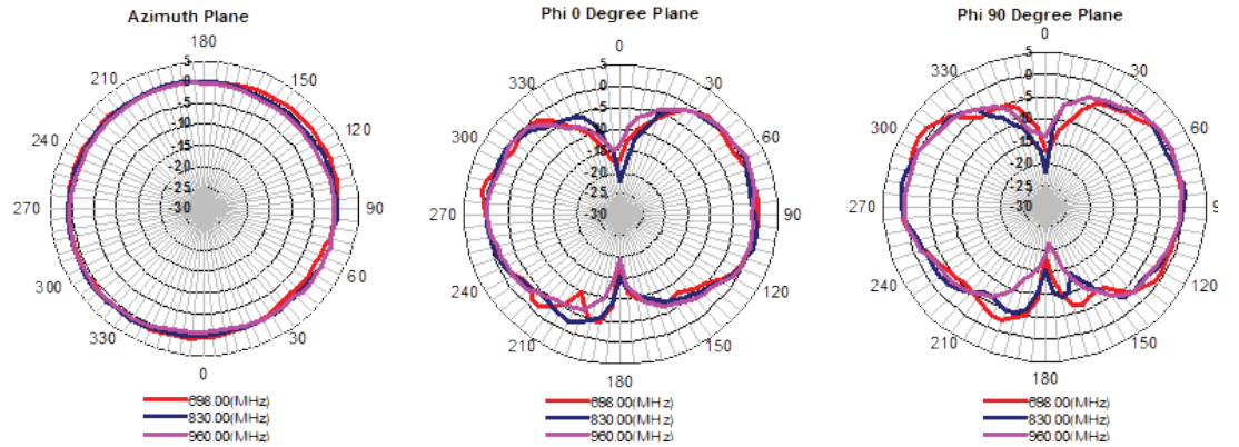
698-960 MHz Band
