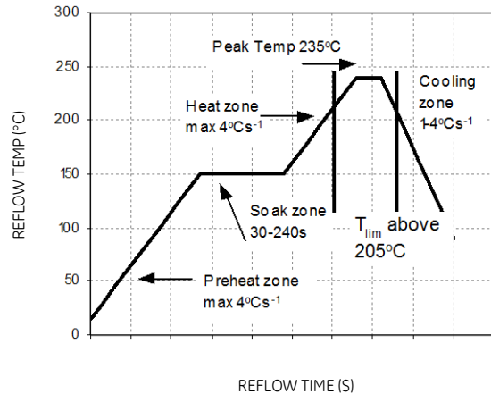
Figure 35. Reflow Profile for Tin/Lead (Sn/Pb) process.
