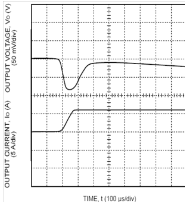
Figure 10. Typical Transient response to Step load change from 0% to 100% of I_{0,\text{max}} at 5V Input.
