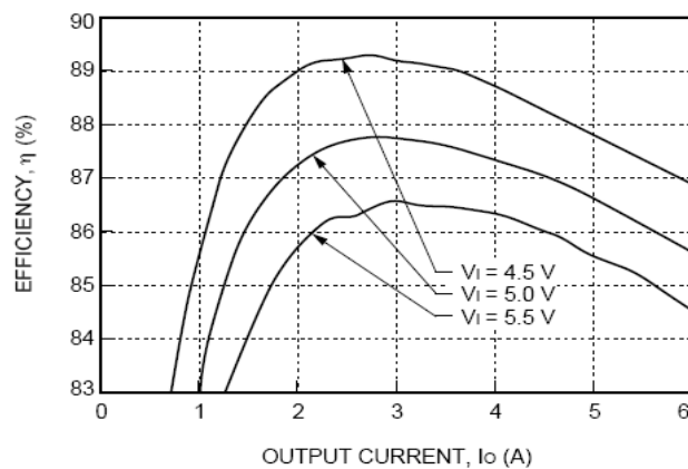
Figure 6. Typical Efficiency for NH020F.
