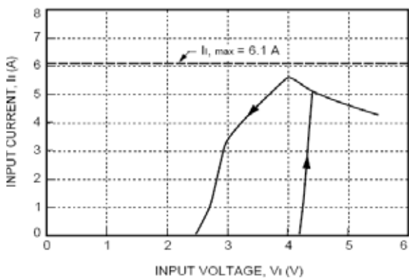
Figure 1. Typical Input Characteristics at 6 A output current.
