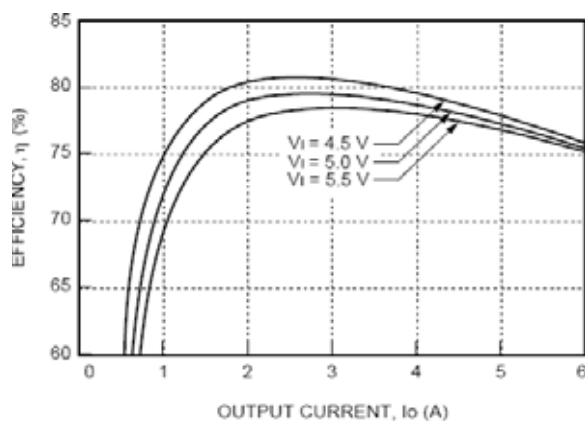
Figure 5. Typical Efficiency for NH020A0G.
