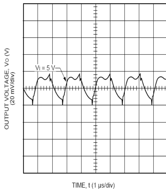
Figure 9. Typical Output Ripple Voltage for NH020F,G (6A Output Current).
