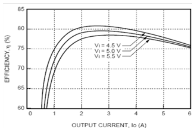
Figure 4. Typical Efficiency for NH020Y.
