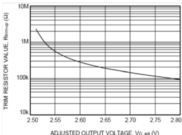
Figure 25. NH020G Rtrim-up Test Results .
