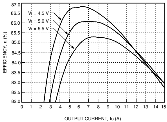
Figure 20. NH050S1R8-L Efficiency, T_A = 25^\circ\text{C}
