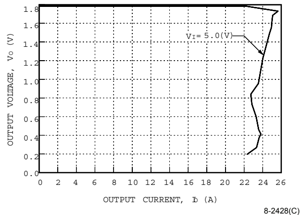
Figure 12. NH050S1R8-L Current Limit, T_A = 25\text{ }^{\circ}\text{C}
