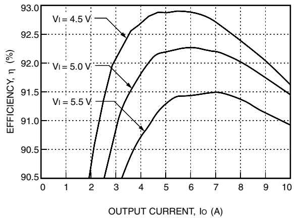
Figure 23. NH033F-L Efficiency, T_A = 25^\circ\text{C}
