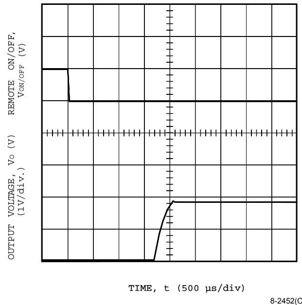
Figure 28. NH050S1R8-L Typical Start-Up from Remote On/Off, V_I = 5\text{ V} , I_O = 15\text{ A}
