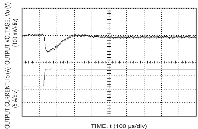
Figure 23. Transient Response to Step Increase in Load from 50% to 75% of Full Load ( V_I = 48 Vdc).
