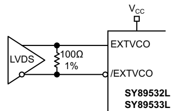
Figure 5h. LVDS
