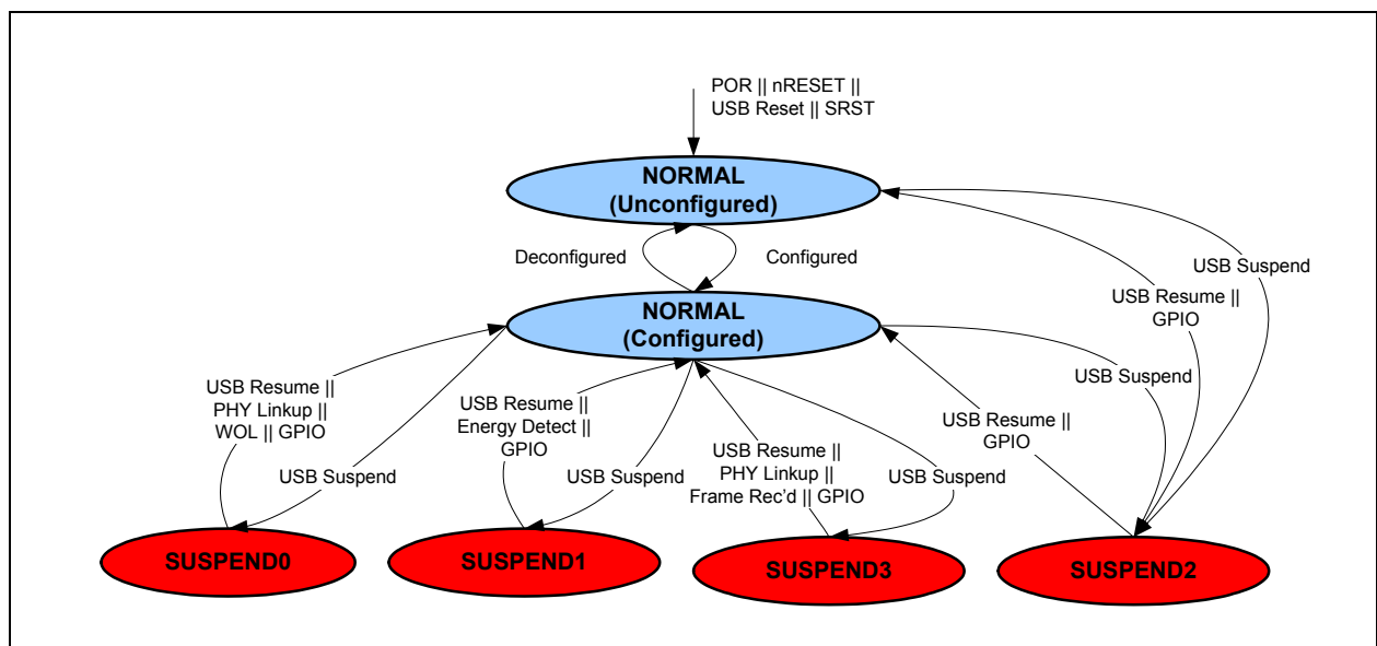
FIGURE 4-29: POWER STATES
