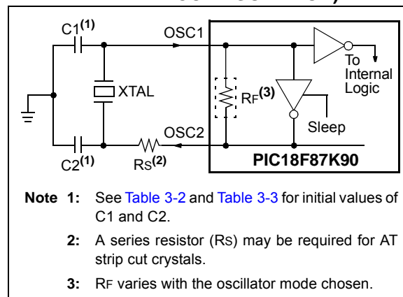
FIGURE 3-2: CRYSTAL/CERAMIC RESONATOR OPERATION (HS OR HSPLL CONFIGURATION)
