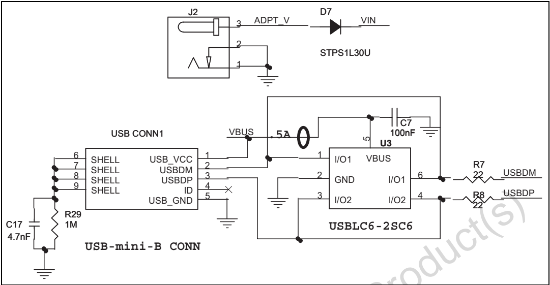
Figure 3. Power supply
