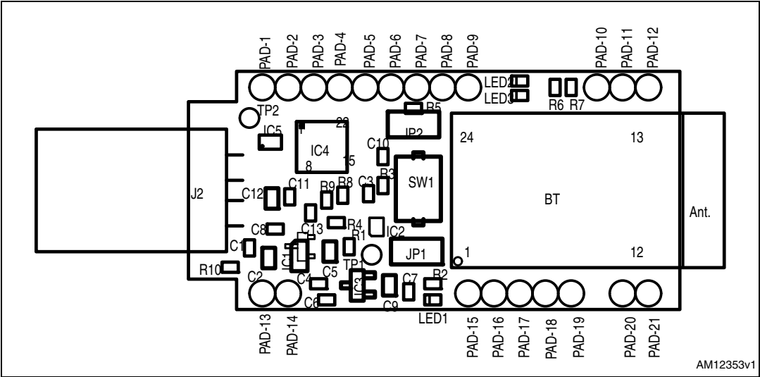
Figure 1. Dongle component layout, front side
