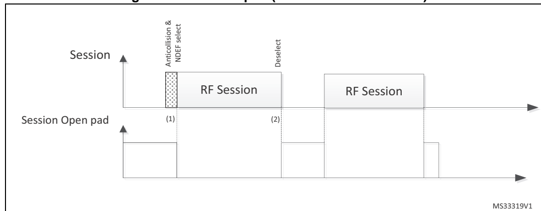
Figure 3. Session Open (RF Session field = 0x11)
