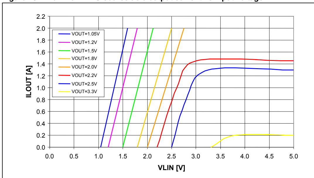
Figure 46. Maximum LDO source able output current vs input voltage
