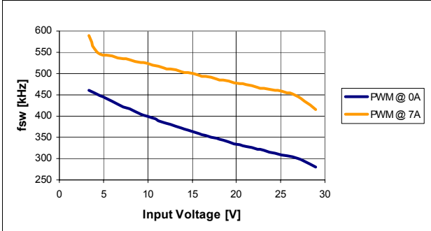
Figure 13. Switching frequency vs input voltage, 1.5 V
