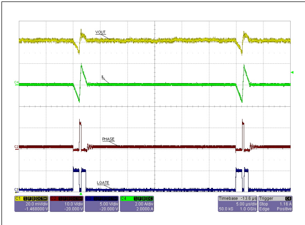
Figure 17. No-audible pulse-skip waveforms
