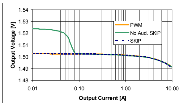
Figure 5. VOUT load regulation, 1.5 V, Vin = 12 V
