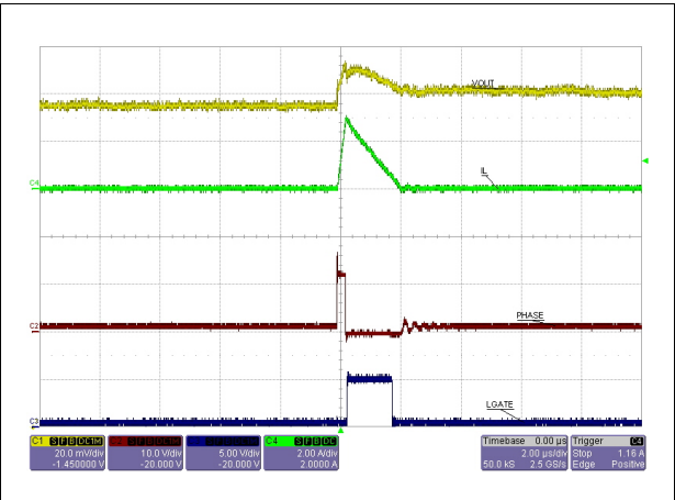
Figure 18. Pulse-skip waveforms
