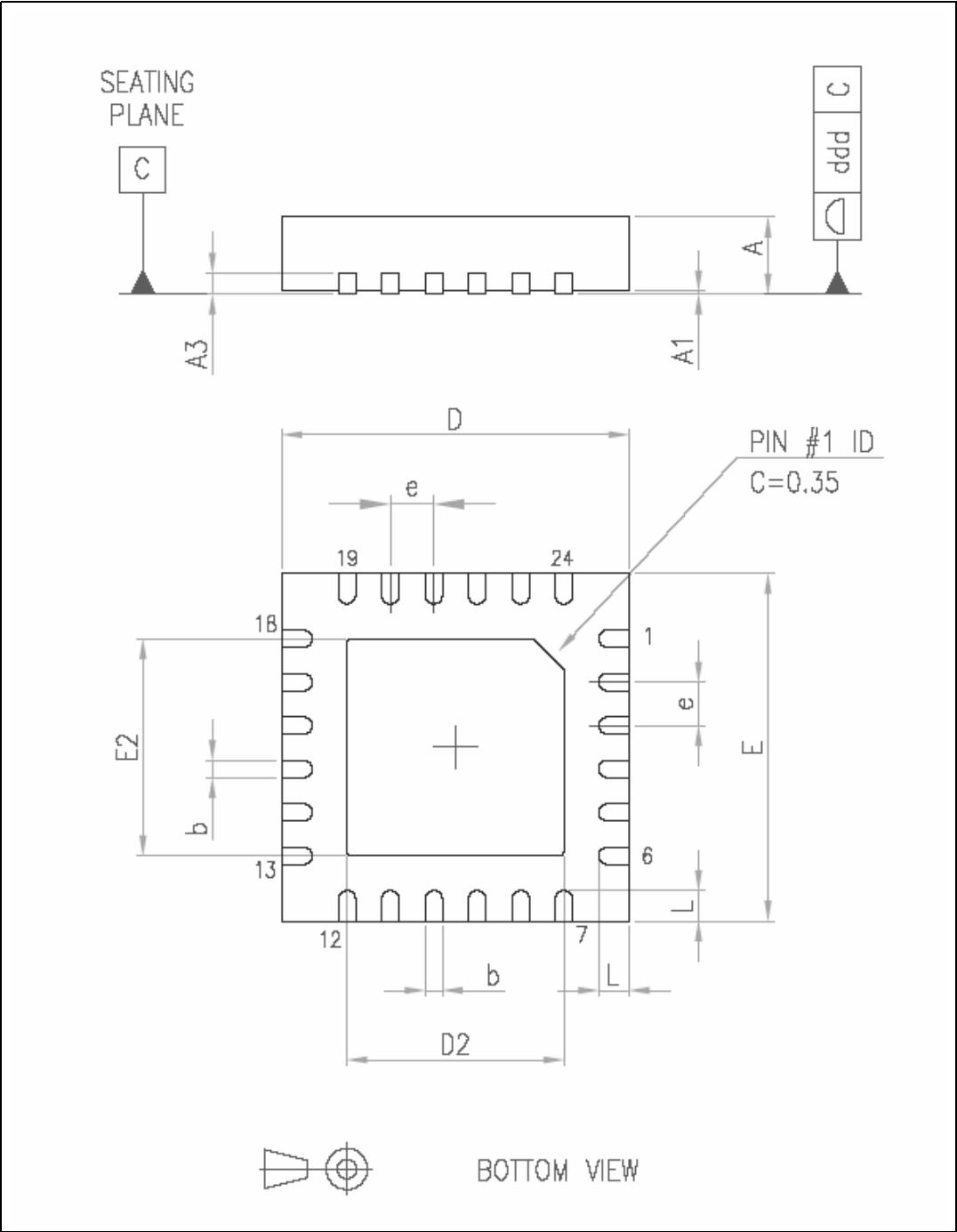
Figure 51. Package dimensions
