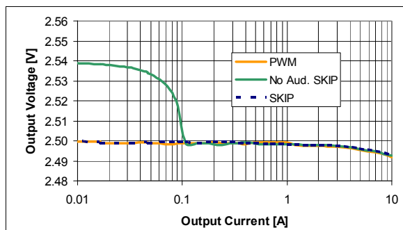
Figure 7. VOUT load regulation, 2.5 V, Vin = 12 V
