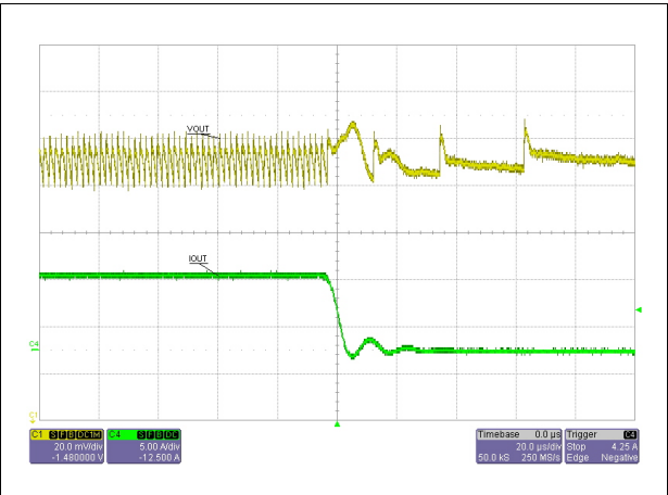
Figure 28. 5 A to 0 A VOUT load transient, Pulse-Skip
