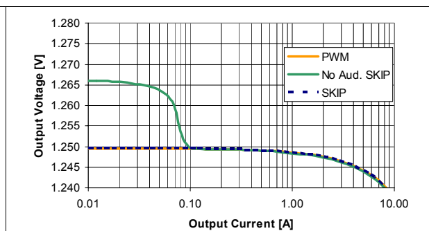
Figure 6. VOUT load regulation, 1.25 V, Vin = 12 V
