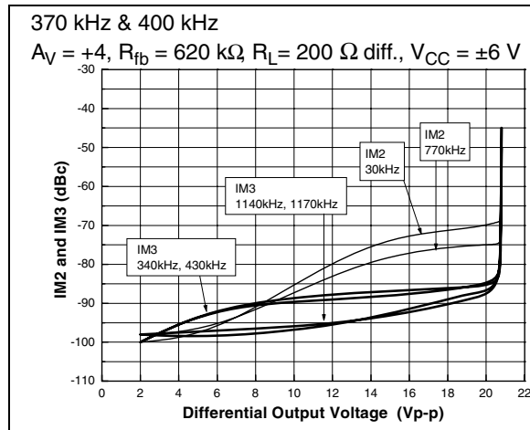
Figure 50. Intermodulation vs. output amplitude
