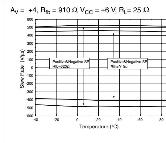
Figure 32. Slew rate vs. temperature
