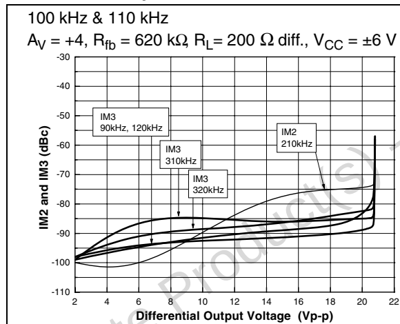
Figure 52. Intermodulation vs. output amplitude
