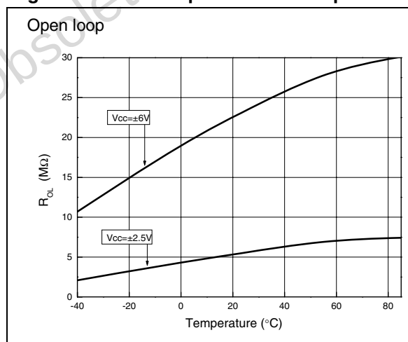
Figure 30. Transimpedance vs. temperature
