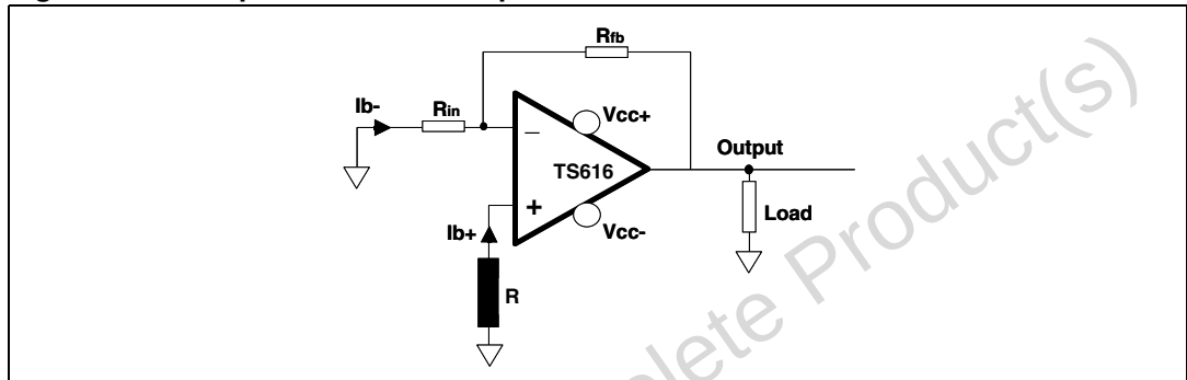
Figure 66. Compensation of the input bias current
