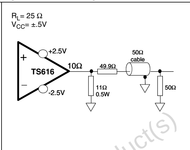
Figure 3. Load configuration
