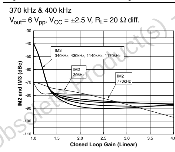
Figure 48. Intermodulation vs. gain
