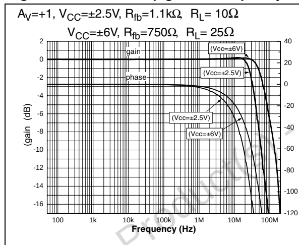
Figure 4. Closed loop gain vs. frequency
