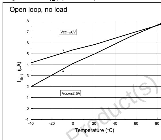
Figure 34. I_{ib}(+) vs. temperature
