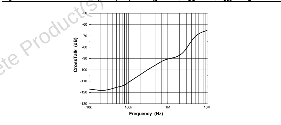
Figure 65. Crosstalk vs. frequency: A_V=+4 , R_{fb}=620\ \Omega , V_{CC}=\pm 6\text{ V} , V_{out}=2\text{ V}_p
