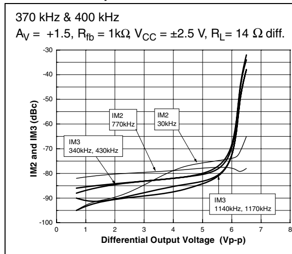
Figure 46. Intermodulation vs. output amplitude
