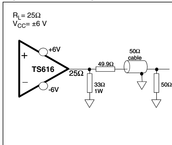
Figure 2. Load configuration
