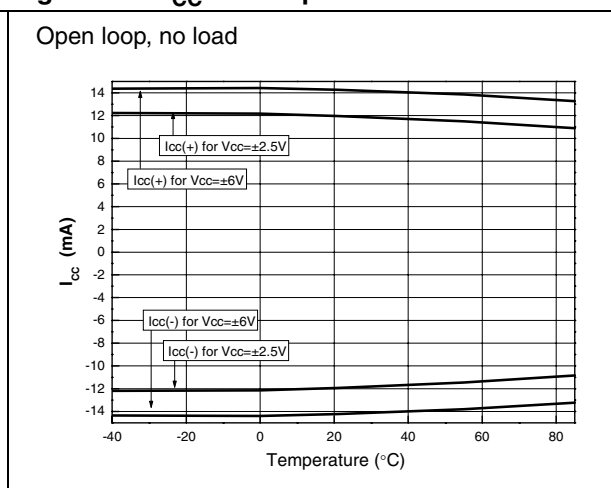
Figure 31. I_{\text{CC}} vs. temperature
