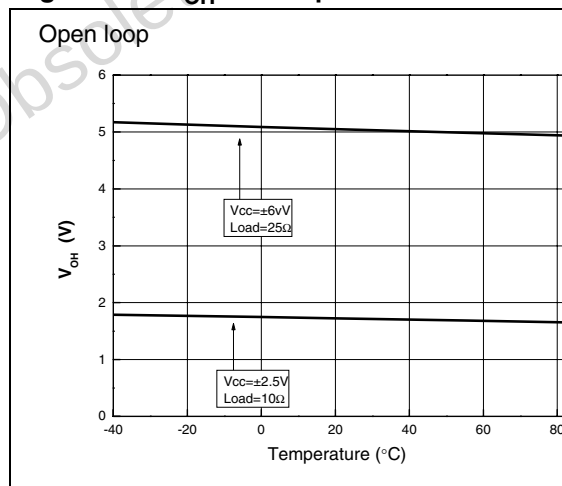
Figure 36. V_{OH} vs. temperature
