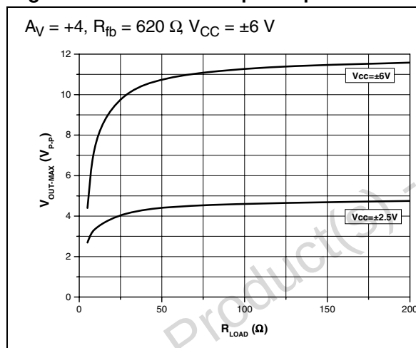
Figure 28. Maximum output amplitude vs. load
