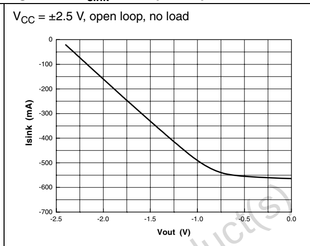
Figure 27. I_{\text{sink}} vs. output amplitude
