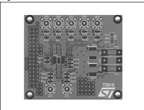
Figure 56. Evaluation board
