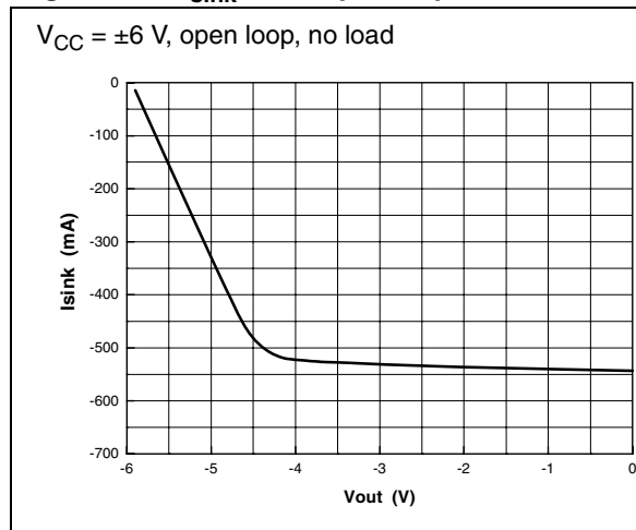
Figure 26. I_{\text{sink}} vs. output amplitude
