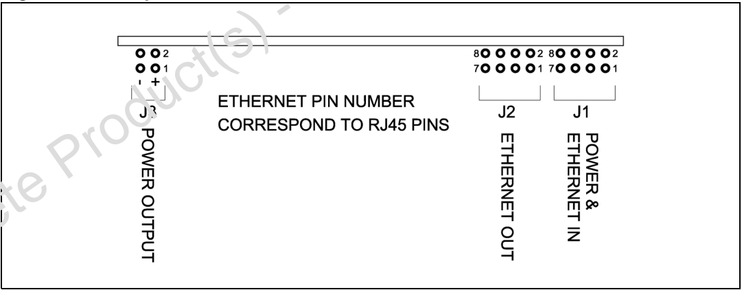
Figure 3. Footprint
