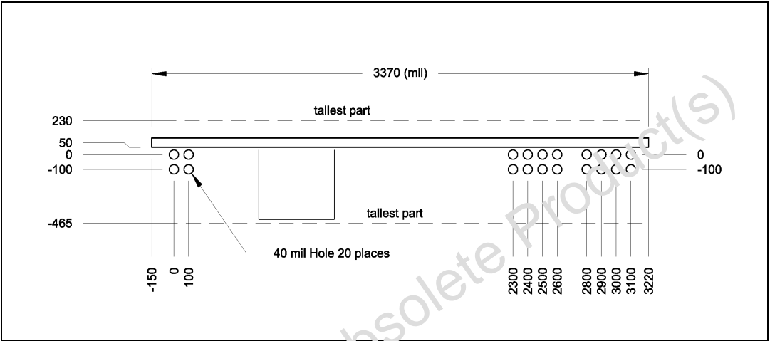
Figure 2. Mechanical dimensions
