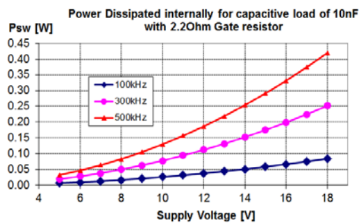
Figure 7. Power dissipation with load of 10 nF and 2.2 \Omega gate resistor
