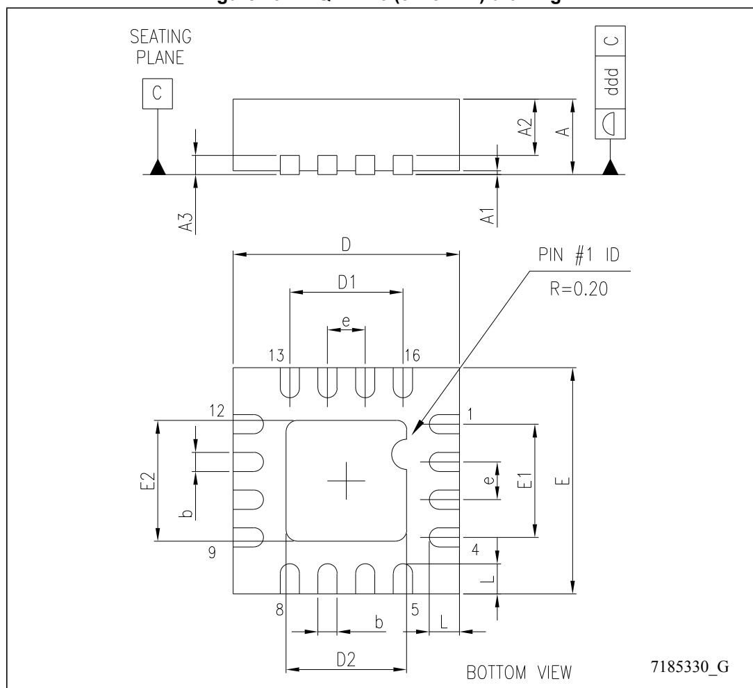
Figure 29. VFQFPN16 (3 x 3 mm) drawing
