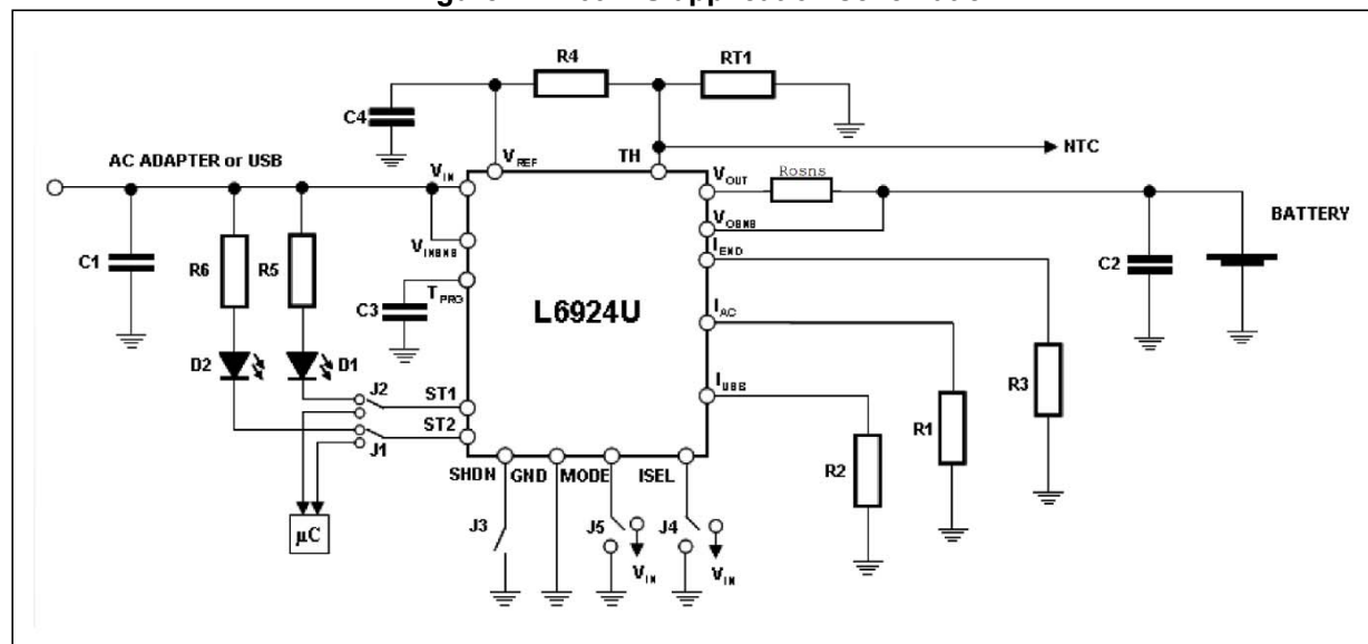
Figure 22. L6924U application schematic
