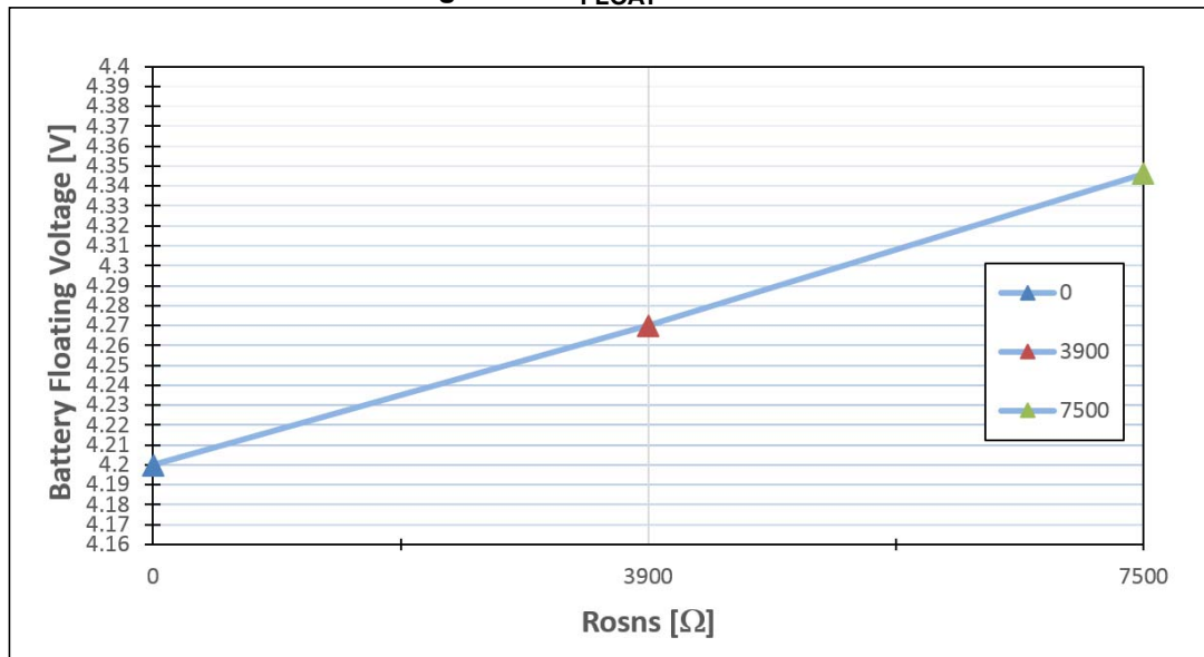
Figure 23. V_{\text{FLOAT}} vs. R_{\text{SNS}}
