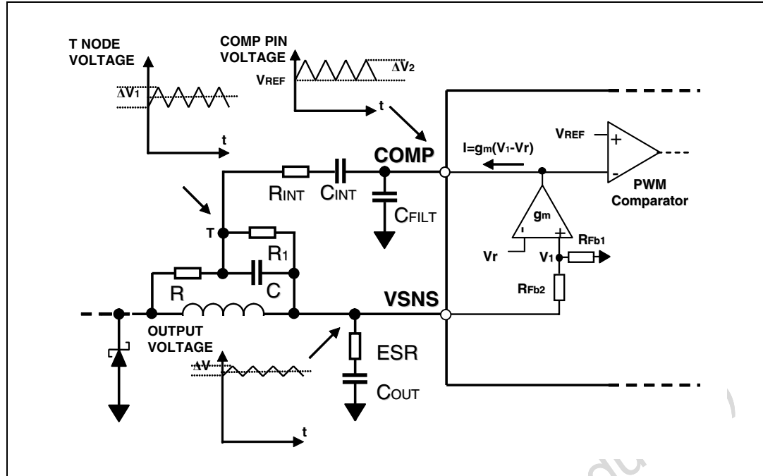
Figure 8. "Virtual-ESR" network
