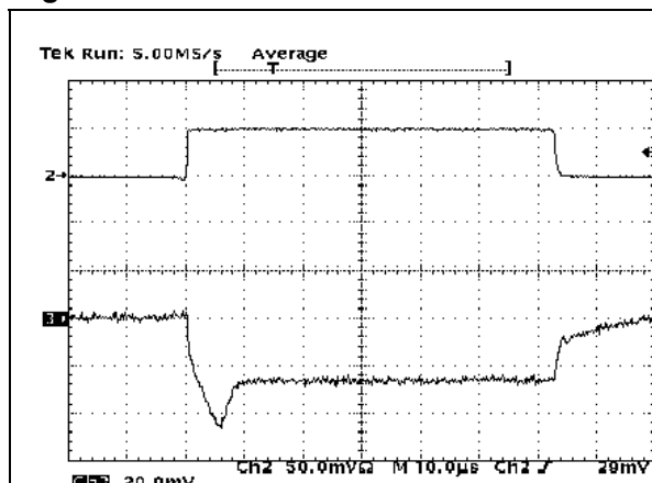
Figure 15. Load transient
