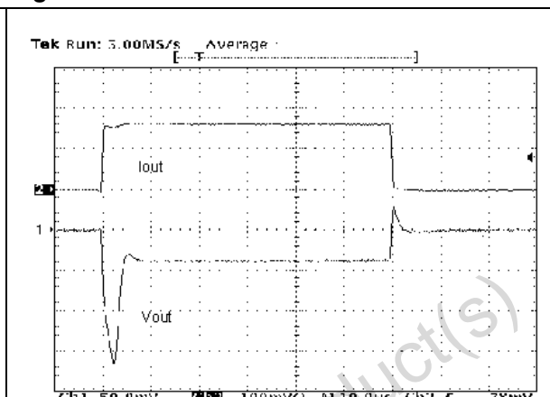
Figure 16. Load transient
