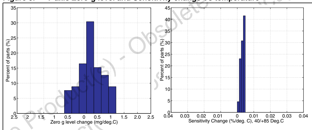
Figure 9. Y-axis Zero-g level and Sensitivity change Vs temperature
