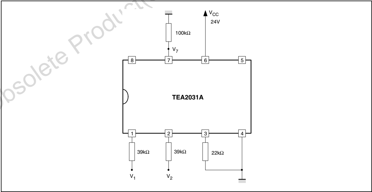
Figure 5. PARABOLA TEST DIAGRAM
