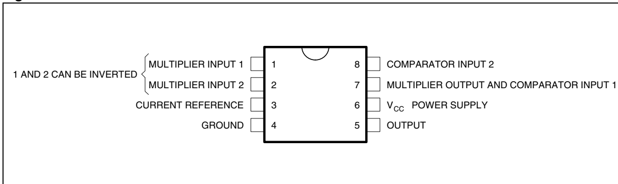
Figure 2. Pin Connections
