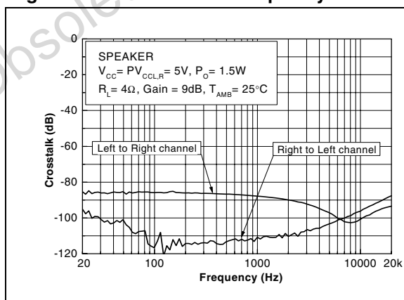
Figure 30. Crosstalk vs. frequency
