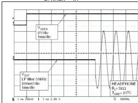
Figure 28. Wake-up time, V_{CC}=PV_{CCL,R}=CPV_{CC}=HPV_{CC}=5V , V_{HDEN}=V_{IL}
