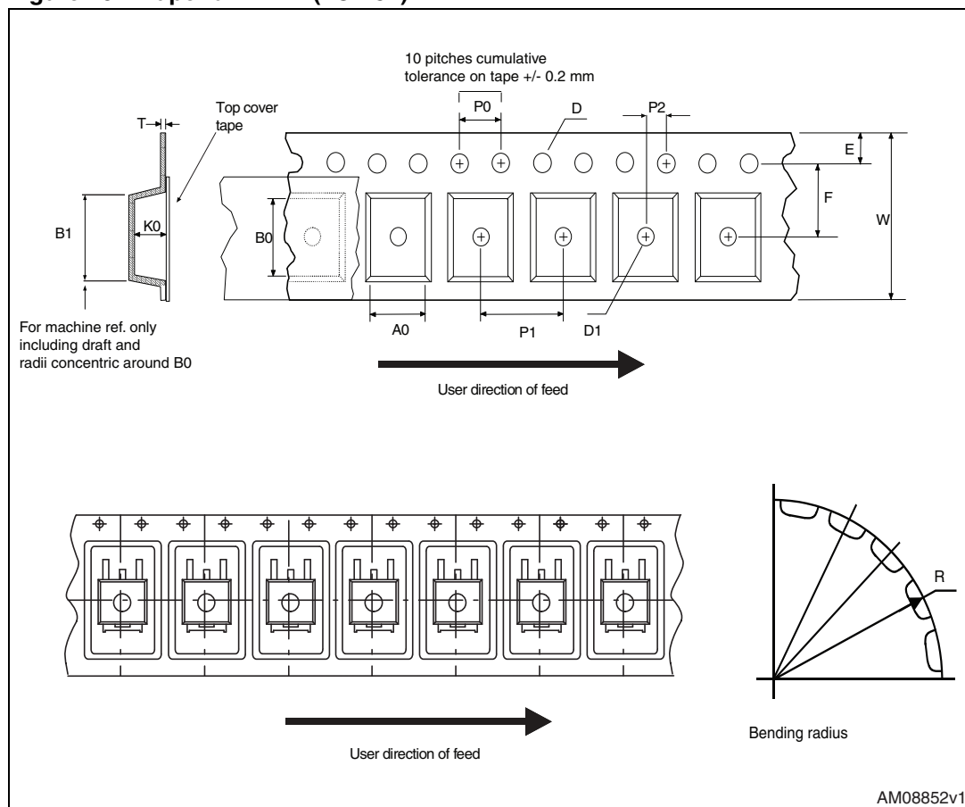
Figure 10. Tape for DPAK (TO-252)
